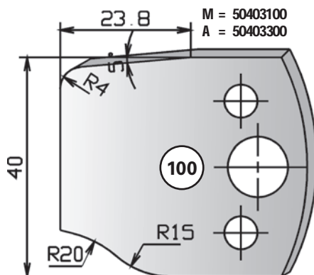
Panel Raising Profile A1 Deflector A1
