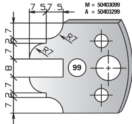
Counter Profiles K1-K4 Deflector K1- K4
