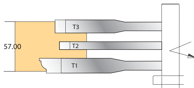
Sash – Combe Joints
