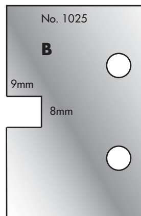
Cutter: 003H01025 Limiter: 004H01025
