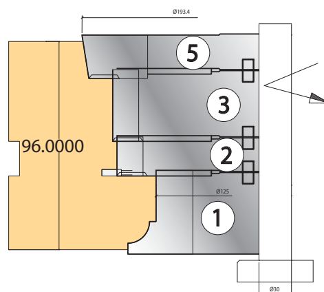
HP flush frame inner tool change
