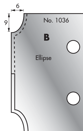
Cutter: 003H01036 Limiter: 004H01036
