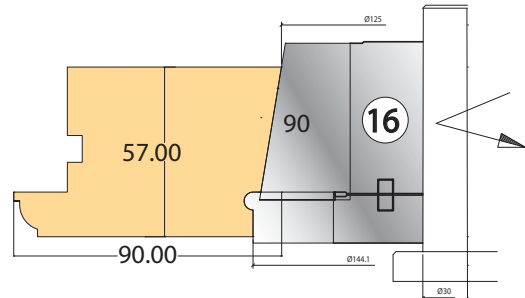
Traditional cill profile
