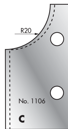
Cutter: 003H01106 Limiter: 004H01106
