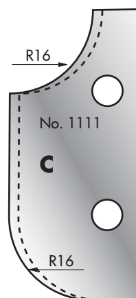
Cutter: 003H01111 Limiter: 004H01111
