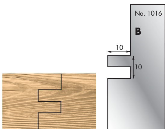
Cutter: 003H01016 Limiter: 004H01016
