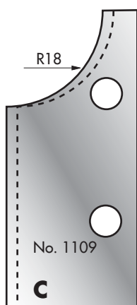
Cutter: 003H01109 Limiter: 004H01109
