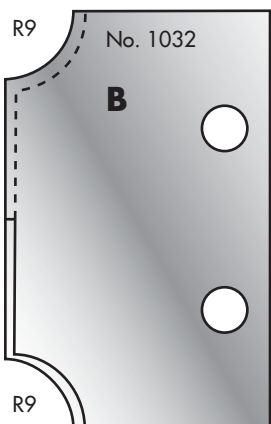
Cutter: 003H01032 Limiter: 004H01032
