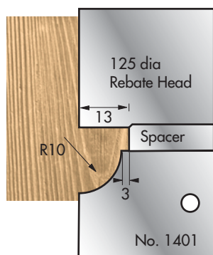
125 dia x 20mm wide 30mm Bore 260S00020 1 1/4 Bore 260S00030
