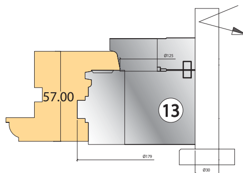
Stormproof outer profile
