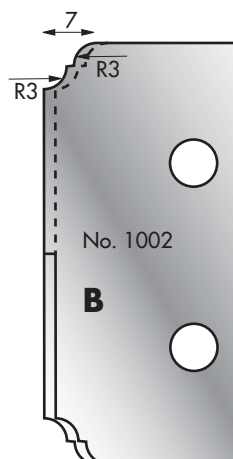
Cutter: 003H01002 Limiter: 004H01002
