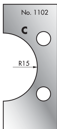
Cutter: 003H01102 Limiter: 004H01102
