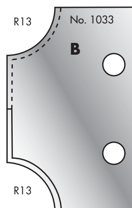
Cutter: 003H01033 Limiter: 004H01033
