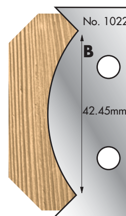
Cutter: 003H01022 Limiter: 004H01022
