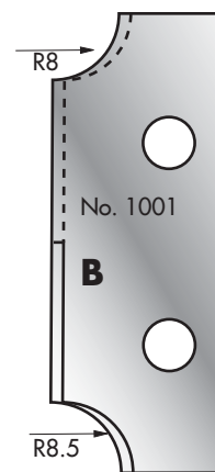
Cutter: 003H01001 Limiter: 004H01001
