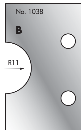
Cutter: 003H01038 Limiter: 004H01038
