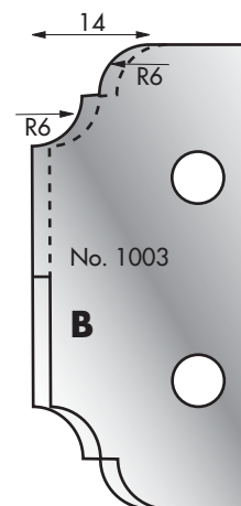
Cutter: 003H01003 Limiter: 004H01003
