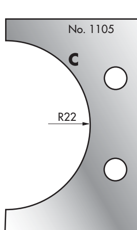
Cutter: 003H01105 Limiter: 004H01105
