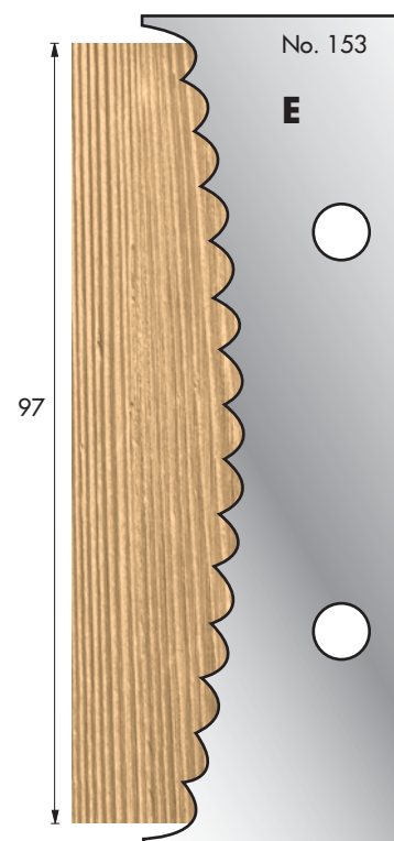
Cutter: 003H00153 Limiter: 004H00153
