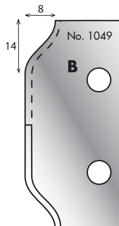
Cutter: 003H01049 Limiter: 004H01049
