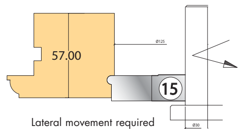
Traditional outer profile
