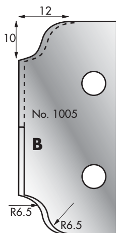
Cutter: 003H01005 Limiter: 004H01005
