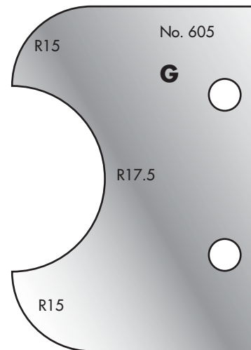
Cutter: 003H00605 Limiter: 004H00605
