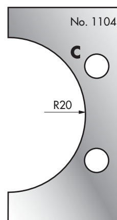
Cutter: 003H01104 Limiter: 004H01104
