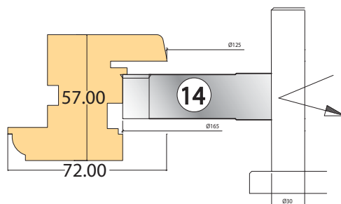
HP Flush outer profile top/bott rail
