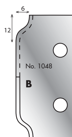
Cutter: 003H01048 Limiter: 004H01048
