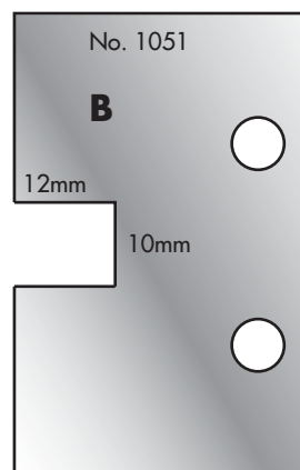
Cutter: 003H01051 Limiter: 004H01051
