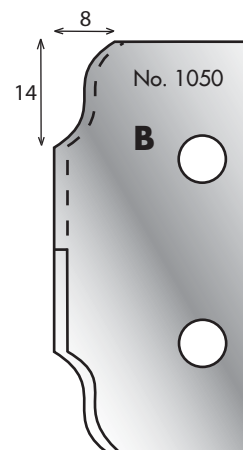
Cutter: 003H01050 Limiter: 004H01050
