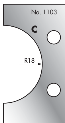
Cutter: 003H01103 Limiter: 004H01103
