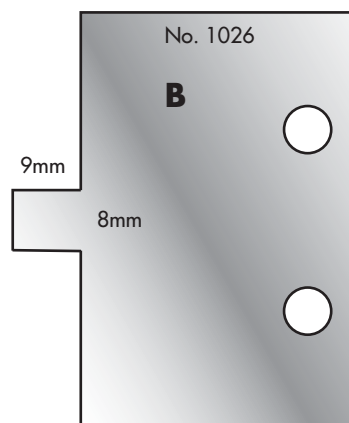
Cutter: 003H01026 Limiter: 004H01026
