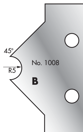
Cutter: 003H01008 Limiter: 004H01008
