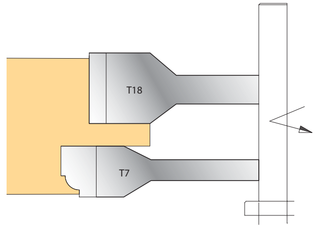
Traditional Frame Tenon – Head
