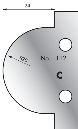
Cutter: 003H01112 Limiter: 004H01112
