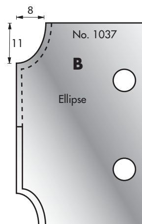
Cutter: 003H01037 Limiter: 004H01037
