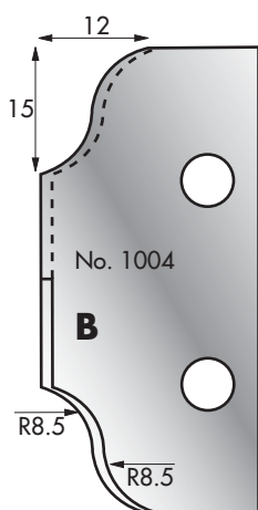
Cutter: 003H01004 Limiter: 004H01004
