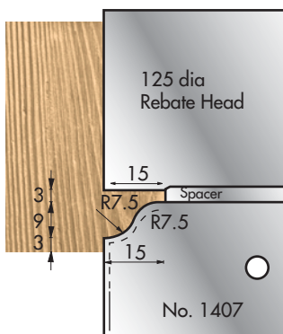
125 dia x 20mm wide 30mm Bore 260S00190 1 1/4 Bore 260S00200
