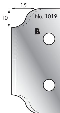
Cutter: 003H01019 Limiter: 004H01019
