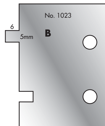
Cutter: 003H01023 Limiter: 004H01023
