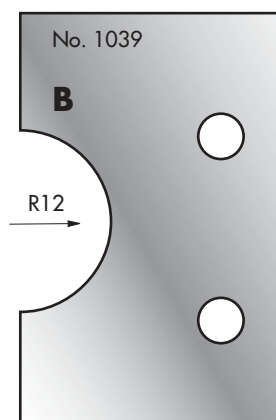
Cutter: 003H01039 Limiter: 004H01039
