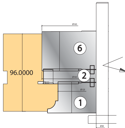
Traditional frame inner head and jambs
