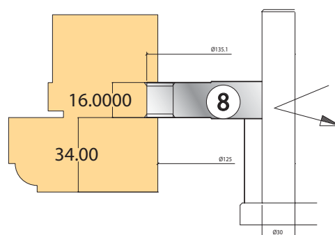
Frame outer all systems
