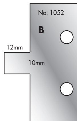
Cutter: 003H01052 Limiter: 004H01052
