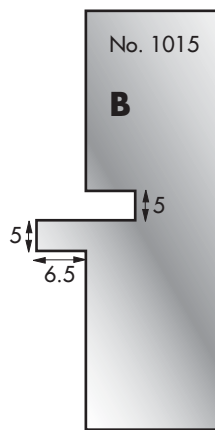
Cutter: 003H01015 Limiter: 004H01015
