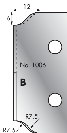
Cutter: 003H01006 Limiter: 004H01006
