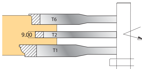
Sash – Combe Joint – Break Joints
