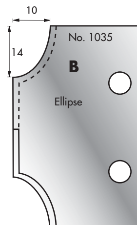
Cutter: 003H01035 Limiter: 004H01035
