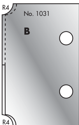
Cutter: 003H01031 Limiter: 004H01031
